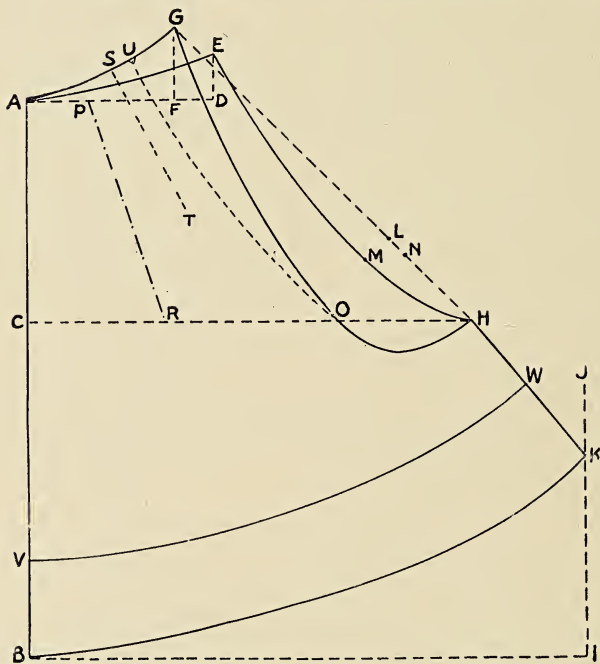
FIG. 62.—Draft of pattern for circular drawers.
